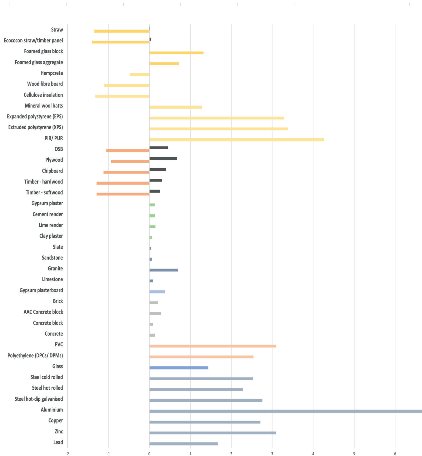
kg CO 2 cradle to gate emissions per kg of material, including sequestration of biobased materials (dark grey - without sequestration)
